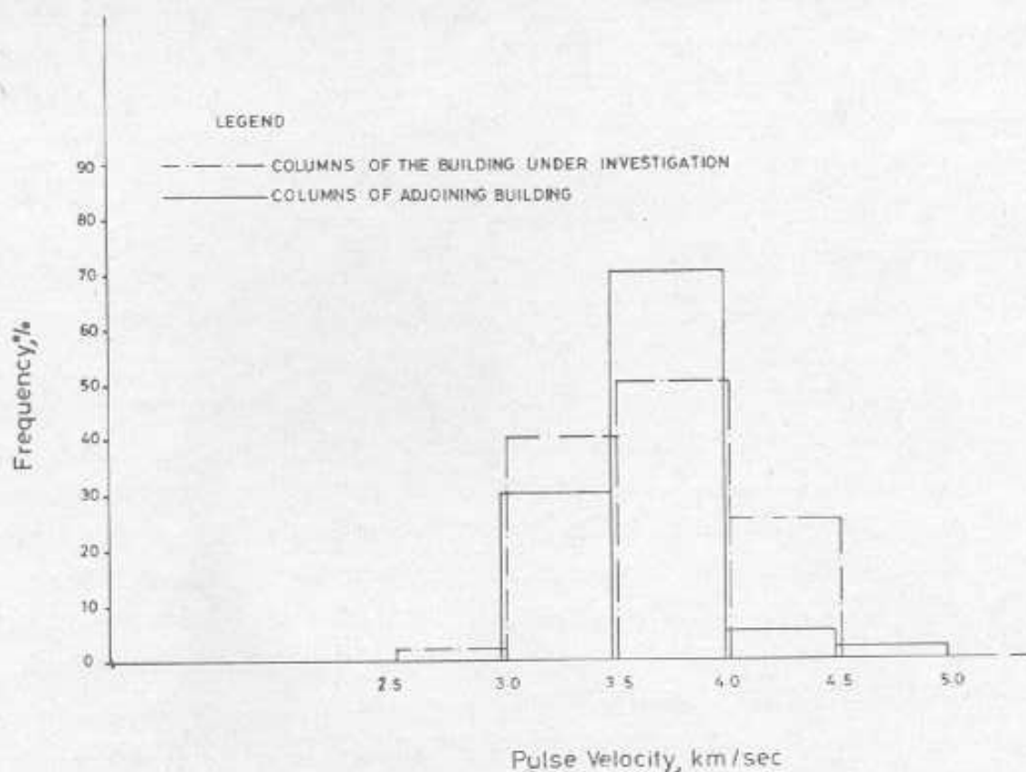
Fig 2 Comparison of pulse velocities in RCC columns
