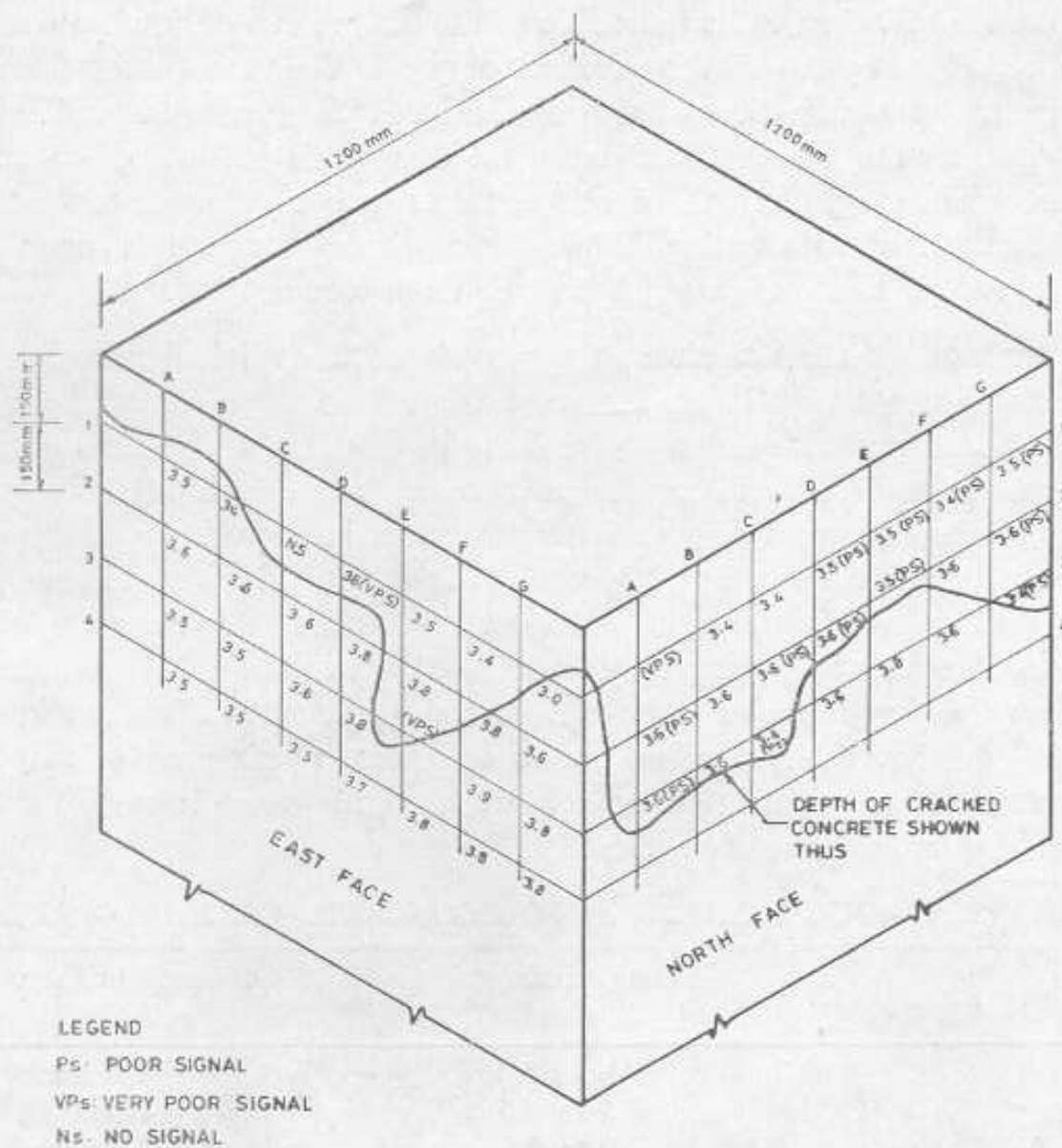
Fig 4 Depth of crack in concrete pedestal as assessed by the ultrasonic pulse velocity measurement
