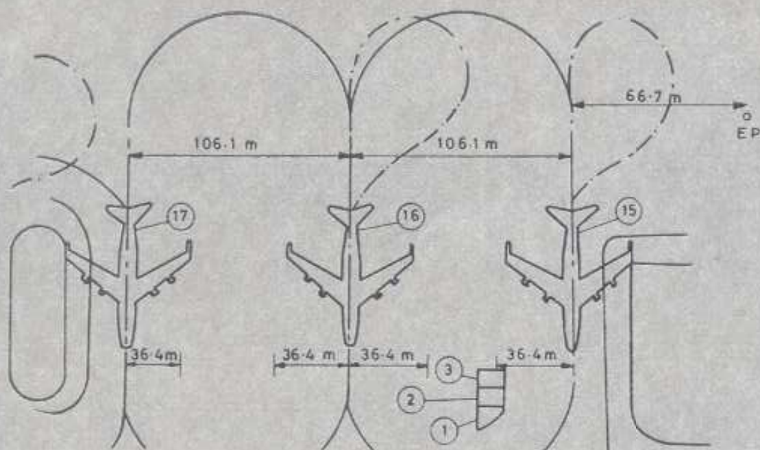
Fig 2 Location of experimental pavements: 1 SFRC full depth; 2 SFRC edge strengthening; 3 PCC
