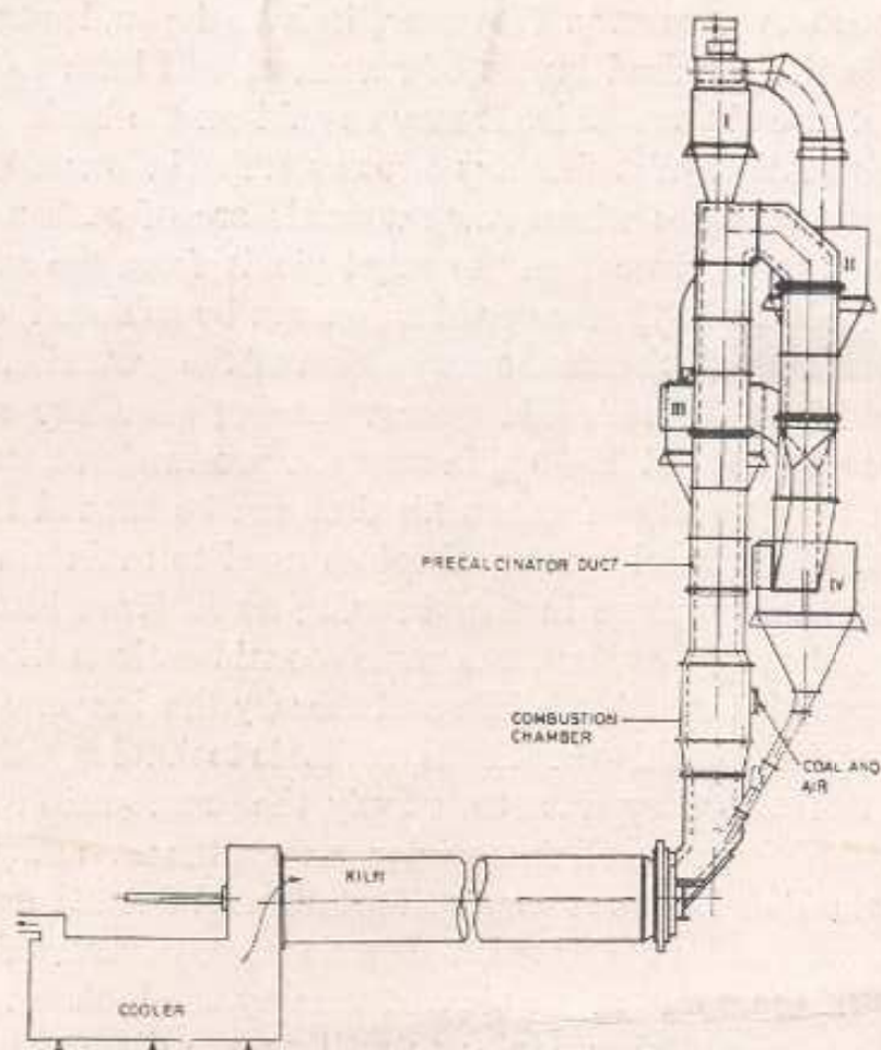
Fig 3 CRI Precal for up to 50% increase in output—System with tertiary air duct
