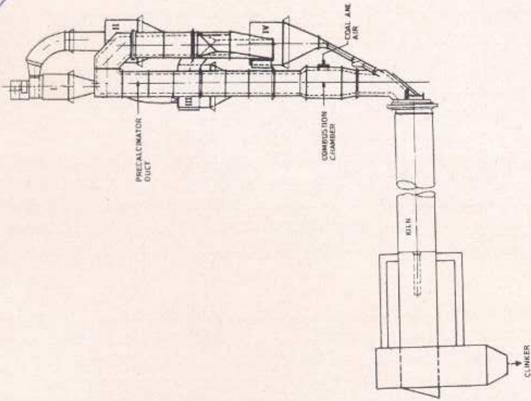
Fig 2 CRI Precal for up to 30% increase in output—System with planetary cooler
