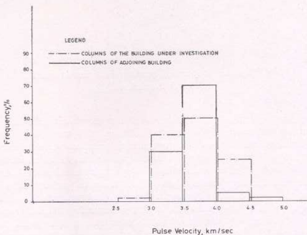
Fig 2 Comparison of pulse velocities in RCC columns
