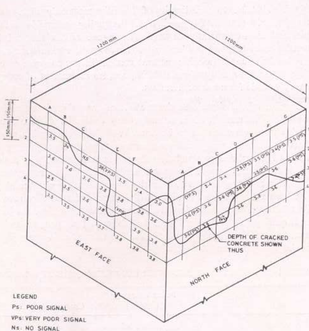
Fig 4 Depth of crack in concrete pedestal as assessed by ultrasonic pulse velocity measurement
